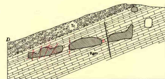
GEOLOGIC MAP AND SECTIONS OF THE SAN ROQUE MINE, HUANCVELICA QUICKSILVER DISTRICT, PERU PLANO Y PERFILES GEOLOGICOS DE LA MINA SAN ROQUE, DISTRITO MERCURIFERO DE HUANCVELICA, PERU
