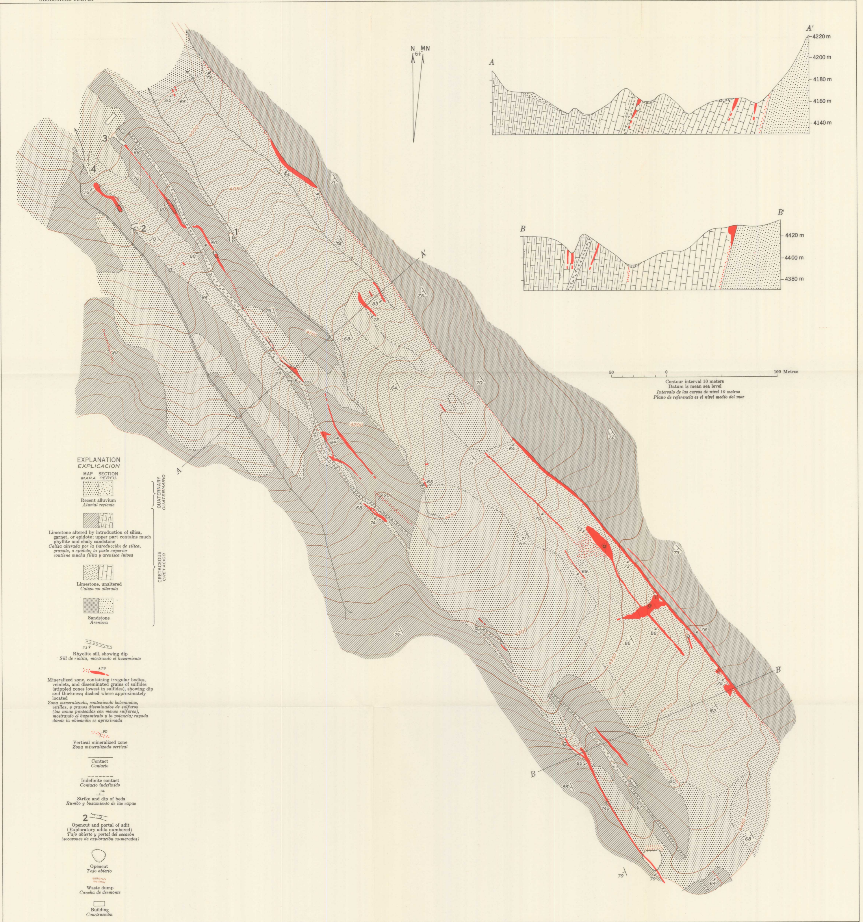
GEOLOGIC AND TOPOGRAPHIC MAP AND SECTIONS OF THE SUSANA MINE, PACLLON-LLAMAC MINING DISTRICT, PERU MAPA GEOLOGICO Y TOPOGRAFICO Y PERFILES DE LA MINA SUSANA, DISTRITO MINERO DE PACLLON-LLAMAC
