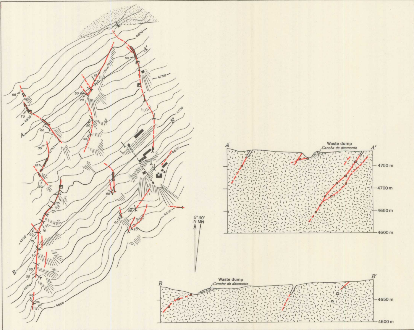
GEOLOGIC MAP AND SECTIONS OF THE HUAMANA MINE, QUEBRADA HONDA-VESUVIO MINING DISTRICT, PERU MAPA GEOLOGICO Y PERFILES DE LA MINA HUAMANA, DISTRITO MINERO QUEBRADA HONDA-VESUVIO
