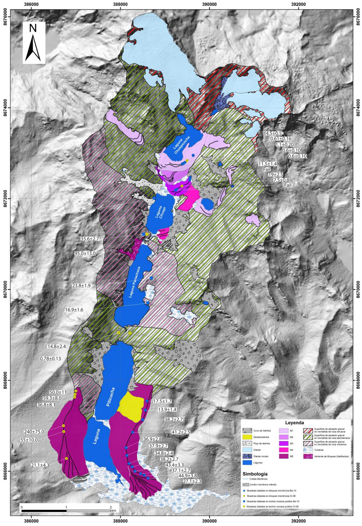
Figure 1. Geomorphological map of the Piticocha Valley - Pariaqaqa Mountain Range
